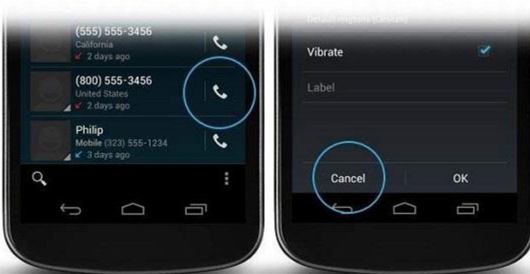
Button Attributes
