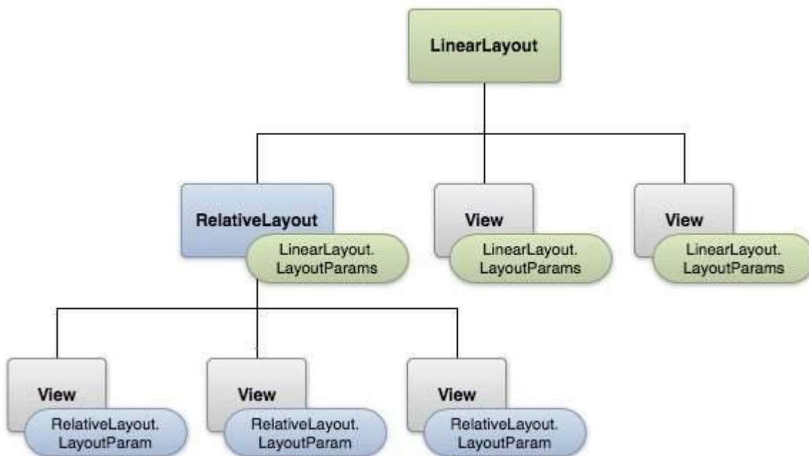
Layout params
